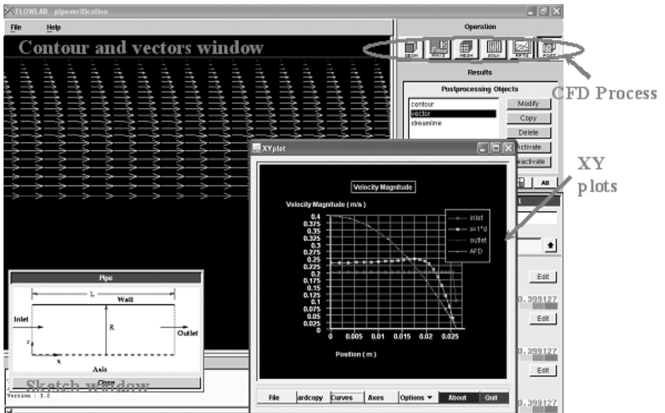
Figure 1. Screen dump for the pipe flow CFD template
