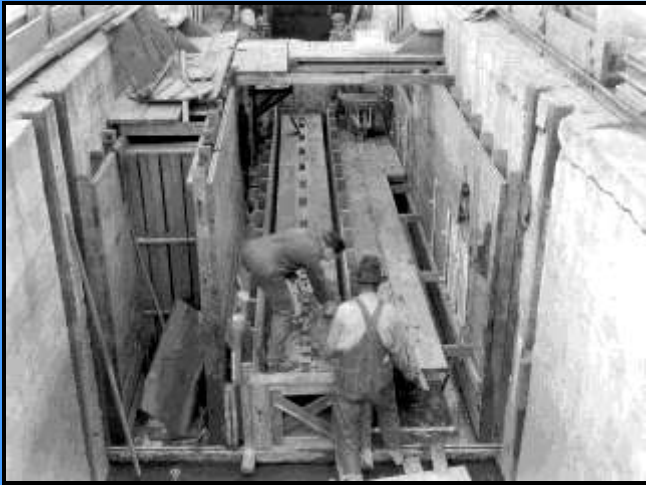
Building a full-scale culvert,
